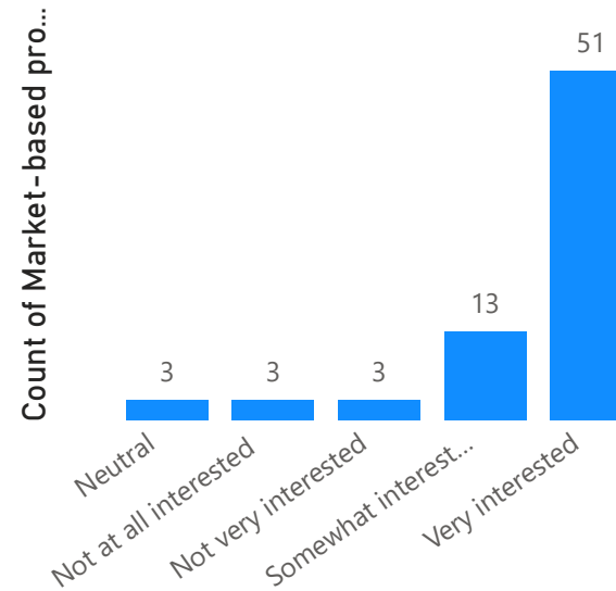
Market-based programming
